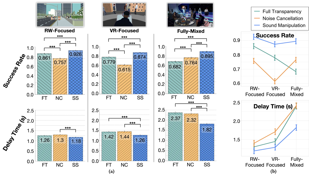
Figure 7: Overall results for RQ3 based on Condition and Scenario, including (a) Success Rate (top, the higher the better) and Delay Time (bottom, the lower the better) with error bars showing 95% confidence intervals. ***= p < 0.0001 . (b) Interaction effects on Success Rate and Delay Time between Condition and Scenario.
